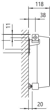
SC single (SCE), type 14 or 16 profile
